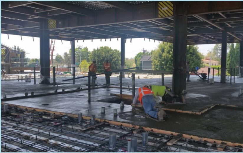
2nd floor deck pour at Area "B"
