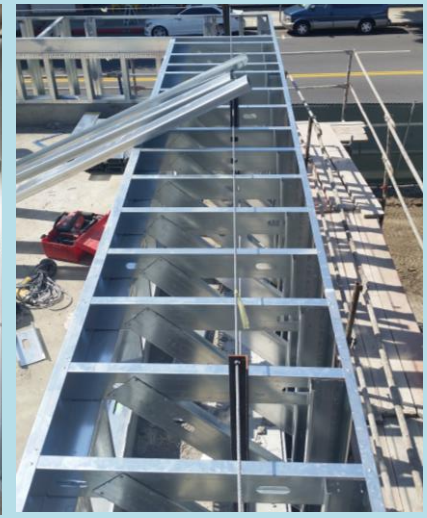
Right - Exterior mtl stud framing for deck parapets.
